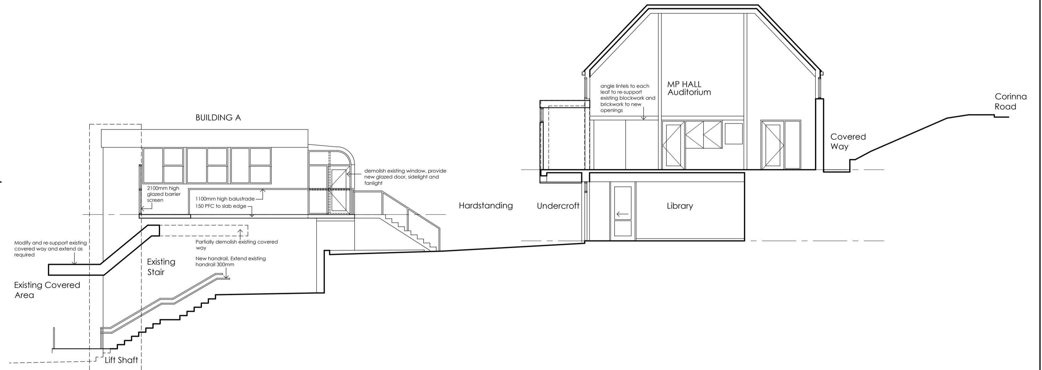
Cross Section
