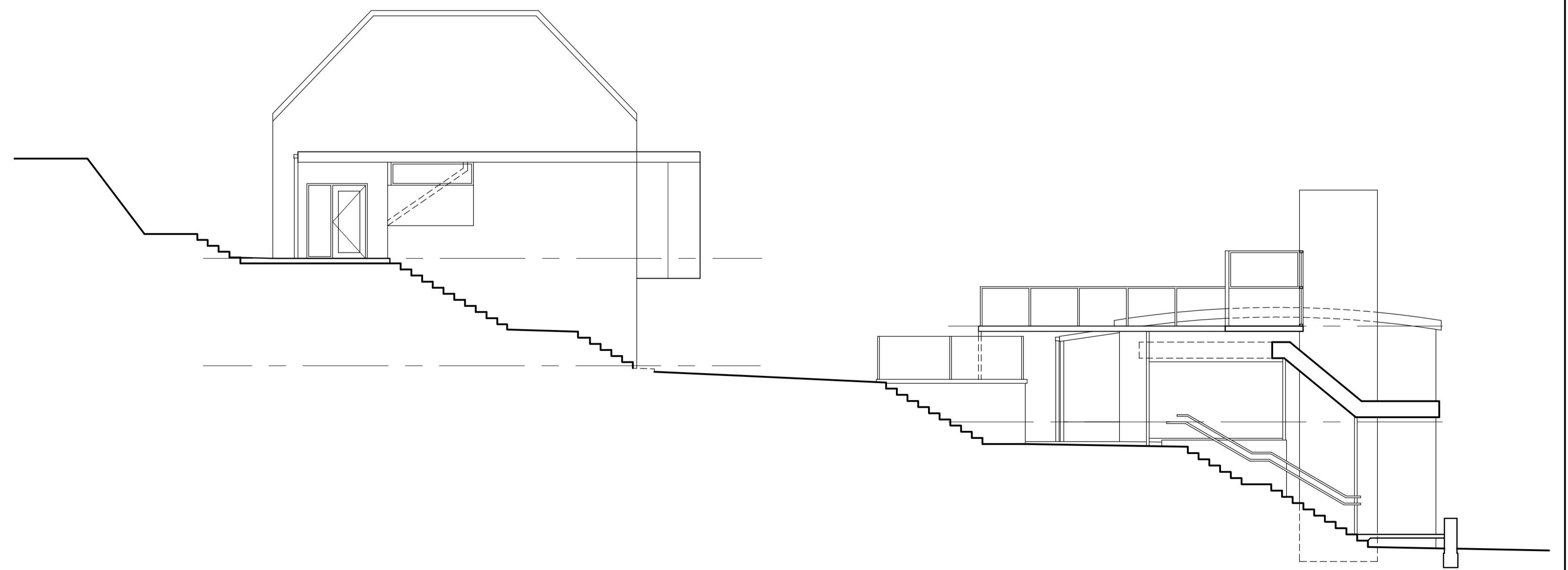
Cross Section
